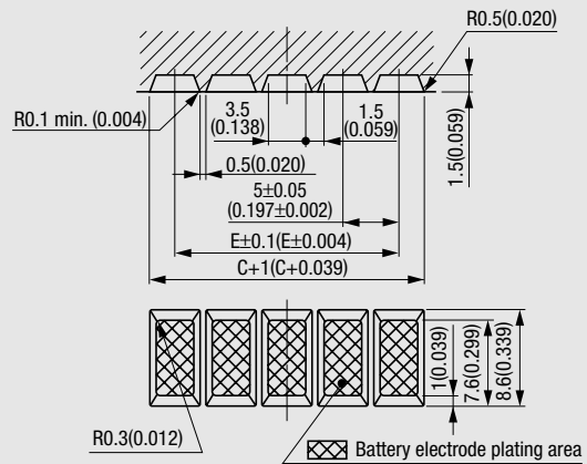
Recommended Dimensions for Battery Terminals
